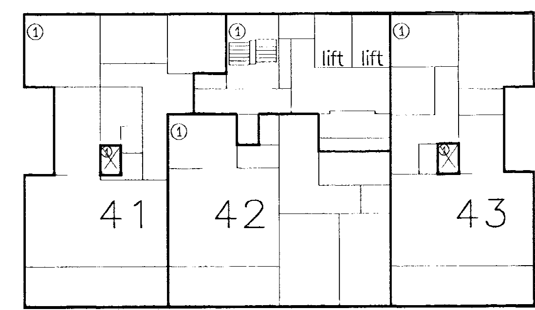
NIVEAU 16 School 1:200
