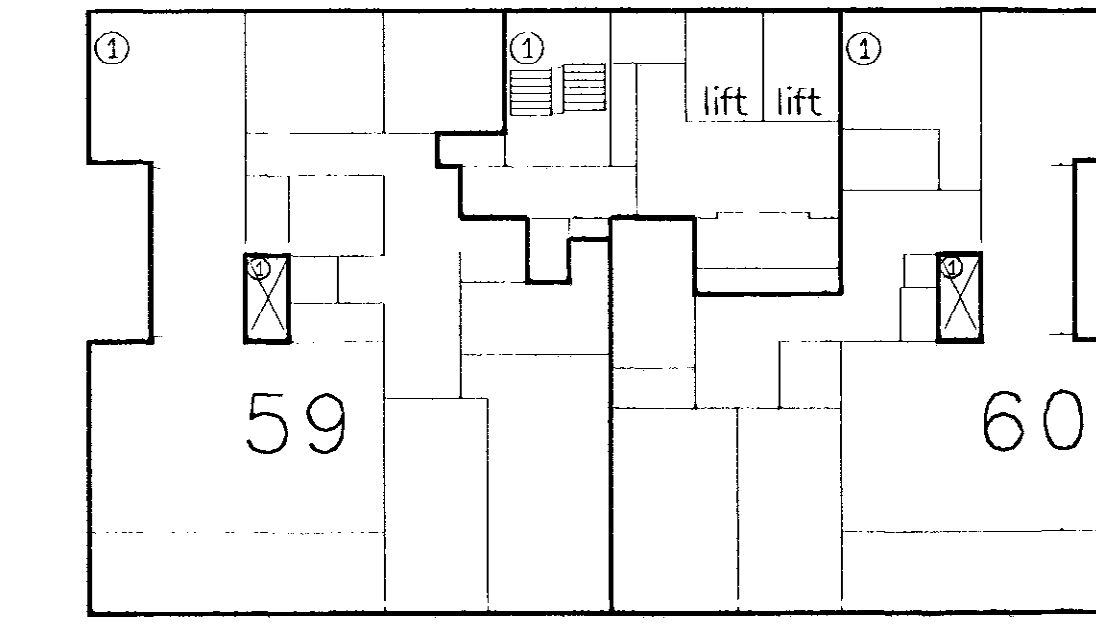
NIVEAU 22 School 1:200
